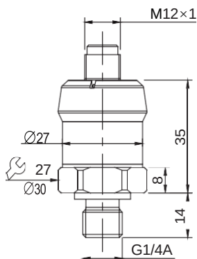
M12×1(4pin) connector
